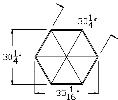
BASE VIEW
