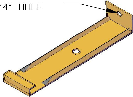
ISO VIEW
