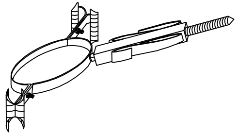
ISO VIEW
