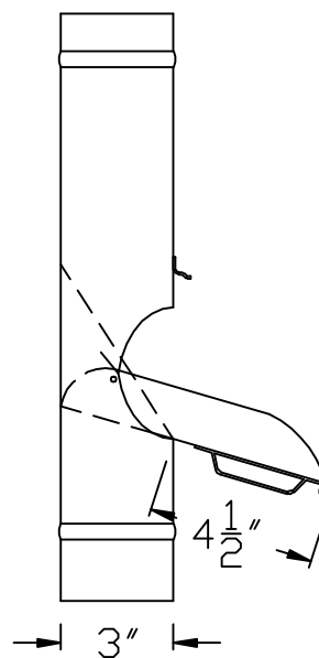
SIDE VIEW
