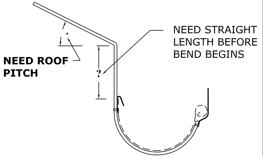
ROOF MOUNTED HR J-HANGER
