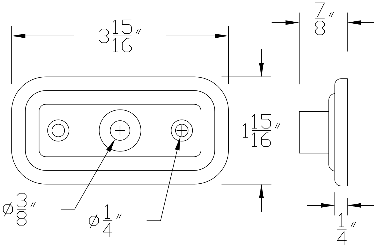
PLAN VIEW
